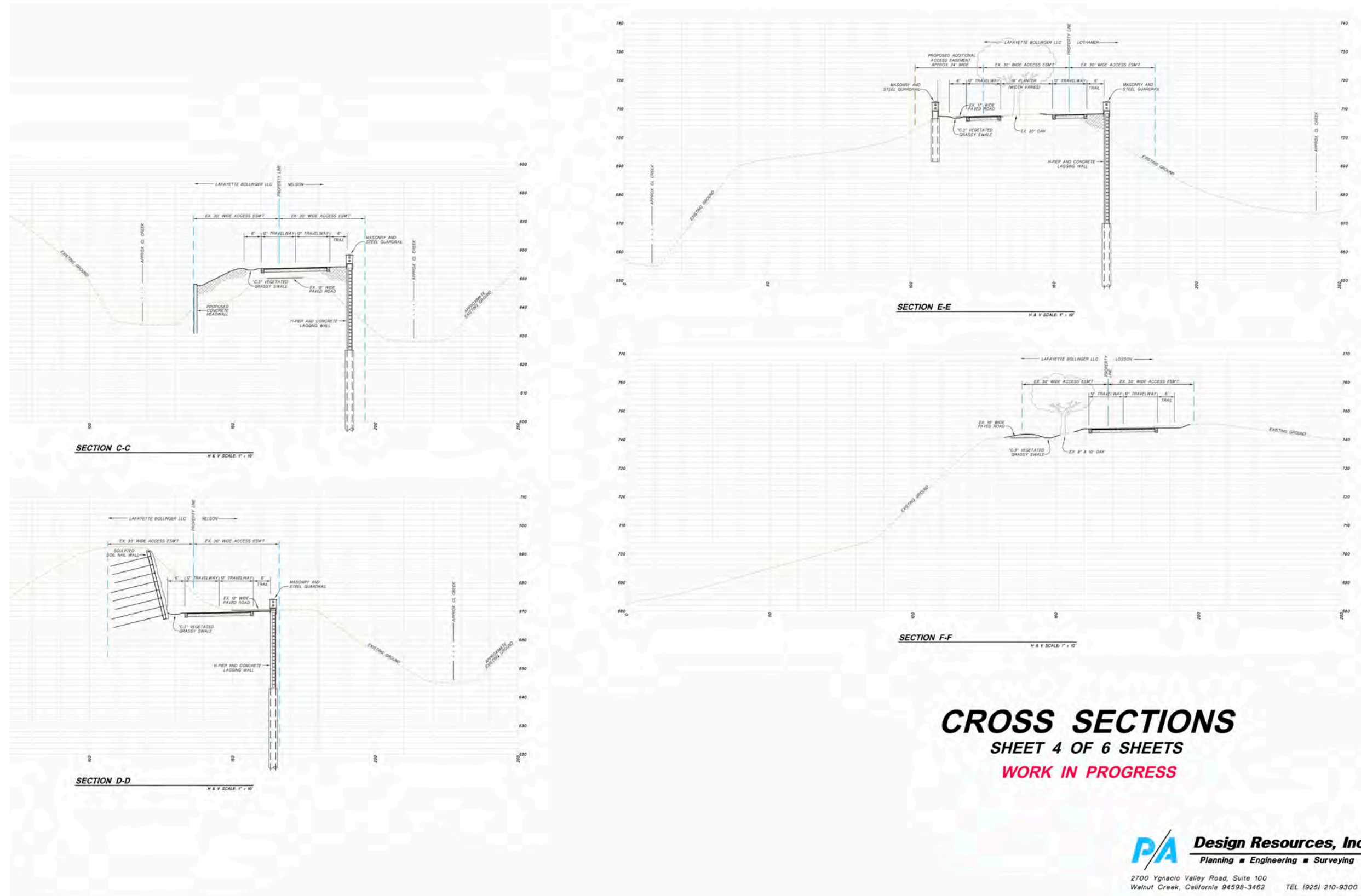
Figure MR7-2: Mitigated Valley Hill Drive Improvement Cross-Sections
