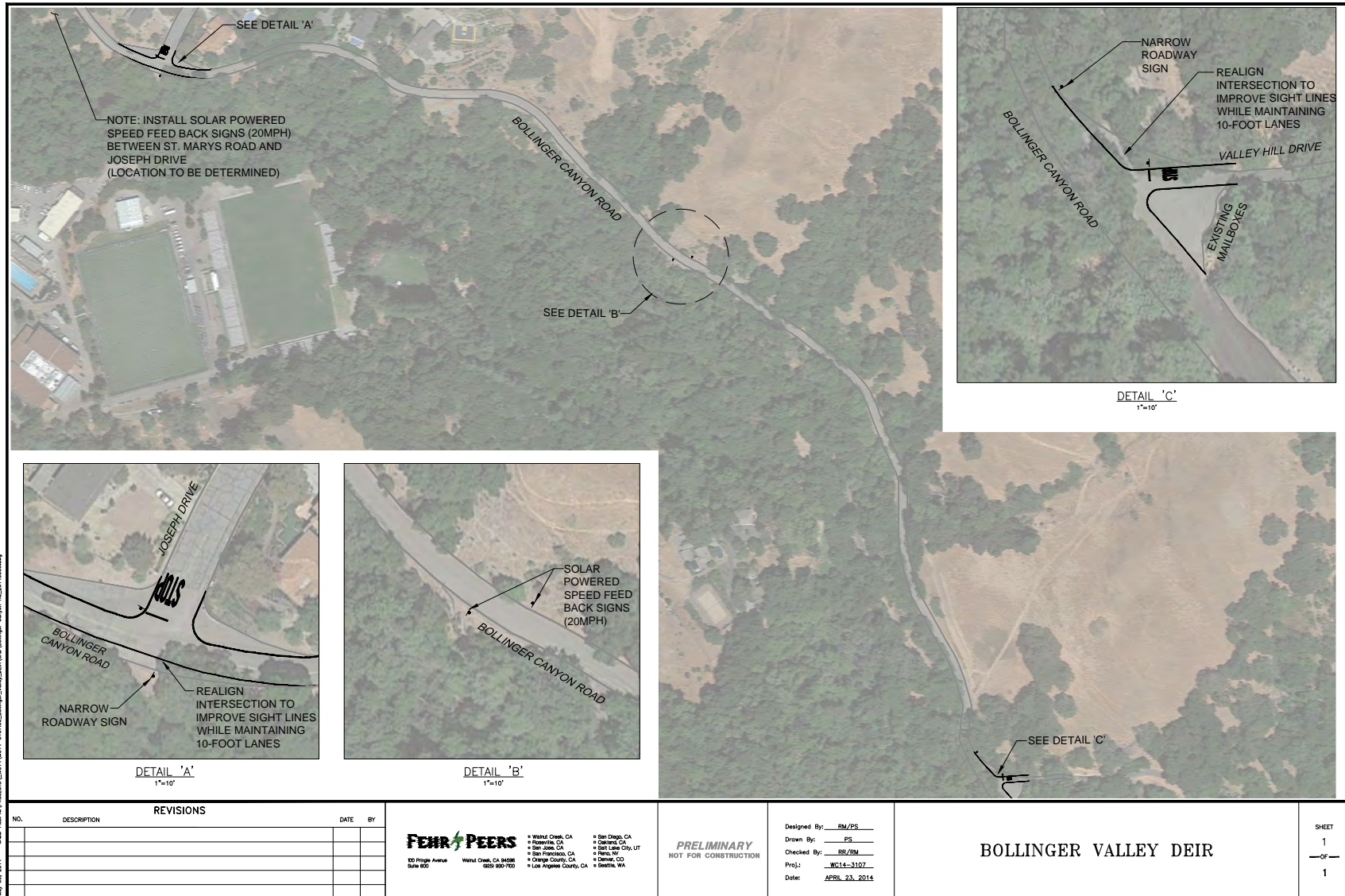
Figure 4.L-3: Proposed Bollinger Canyon Road Improvements
